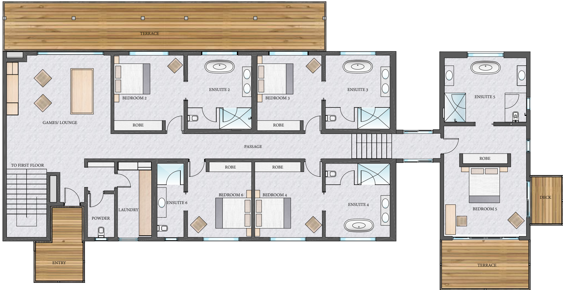
GROUND FLOOR
