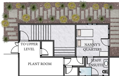
LOWER FLOOR
